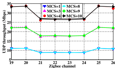
Fig. 4: Impact on 11n throughput for MCSs with same bit rate
