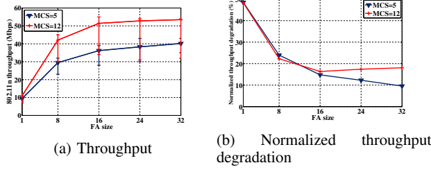
Fig. 14: Throughput of 802.11n at different frame aggregation sizes
