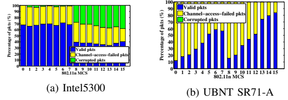
Fig. 6: Packet reception distribution in symmetric scenario
