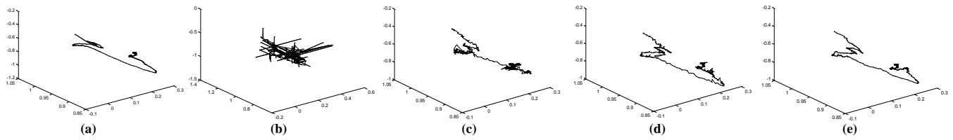
Fig. 6. Comparison results of trajectories (3D positions over time) of joint No.1 (the root joint) of subject 05 sequence 02: (a) ground truth, (b) 20% damaged trajectory, (c) recovered trajectory by [16], (d) recovered trajectory by [17], and (e) recovered trajectory by our method.
